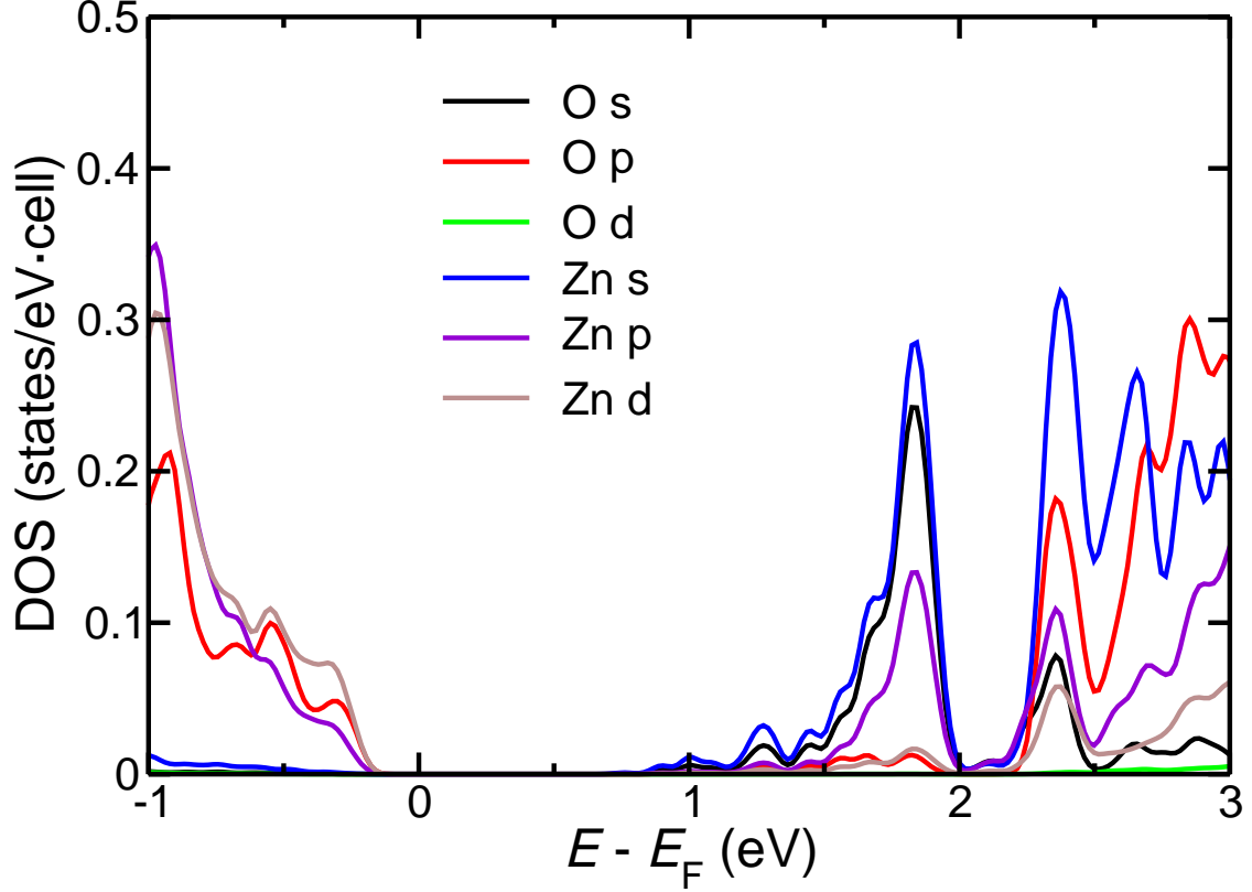
FIG. 2: (Color online) The projected DOS of \text{ZnSe}_{1-x}\text{O}_x with x = 3.125\% .
