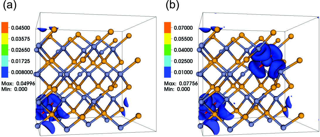
FIG. 1: (Color online) Contour plots of charge density (in units of electron/ \text{\AA}^{-3} ) of \text{ZnSe}_{1-x}\text{O}_x with (a) x = 3.125\% and (b) x = 6.25\% . Max and Min represent the maximum and minimum values of the density within the energy range under consideration. Zn and Se atoms are represented in light blue and orange, respectively, and O atoms are surrounded by the high density region.
