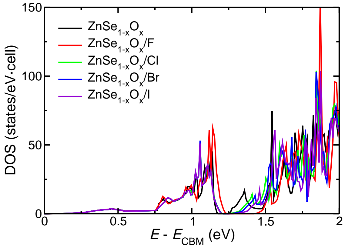
FIG. 3: (Color online) The DOS of ZnSe 1-x O x with halogen dopants.
