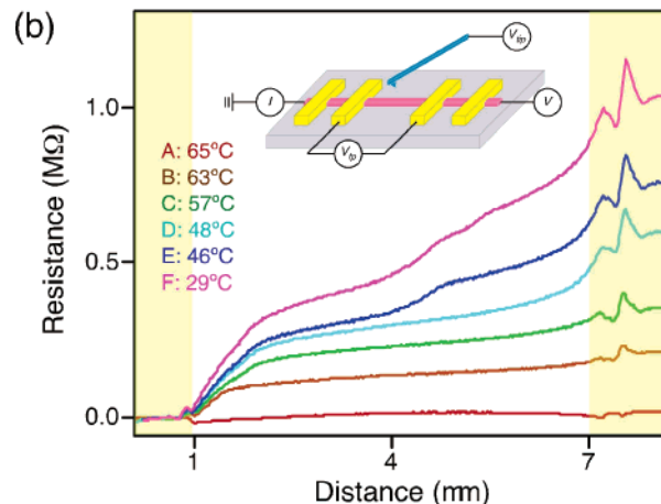
Figure 2. (a) Resistance of an on-substrate VO 2 nanobeam measured in a four-probe geometry as a function of temperature. Red and blue curves are taken during heating and cooling, respectively. Inset, SEM image of the on-substrate VO 2 nanobeam device. The height and width of this nanobeam are 100 and 210 nm, respectively. (b) Resistance profile along the nanobeam length obtained from the same device as in Figure 2a using Kelvin probe microscopy (KPM) at selected temperatures indicated in Figure 2a. The shaded areas on the sides indicate the electrode. On the curves in b, regions with steeper gradient are insulating (I) domains. In curve C, a new I domain appeared at the distance of \sim 1.7\ \mu\text{m} , next to but separated from the existing I domain. Inset, a schematic of KPM applied to a four-probe device. V is the DC bias applied to the nanobeam, I is the current, V_{ip} is the measured four-probe voltage drop between the inner electrodes, and V_{tip} is the voltage applied to the cantilever (the sum of an AC signal at the cantilever resonance frequency and a DC voltage applied by the feedback loop).
